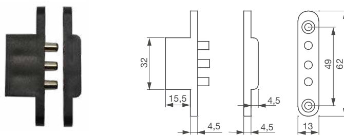
➤ PCT300
