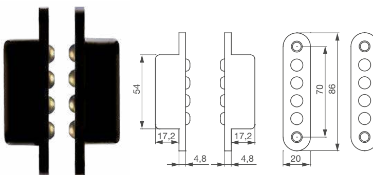
➤ PCT400B
