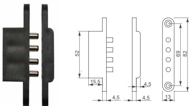
➤ PCT400
