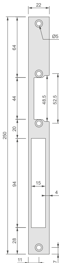
SP25022-F1SUX
