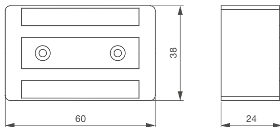
➤ EMS170C
