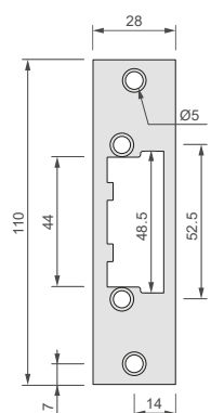
SP11028-U1SUX
