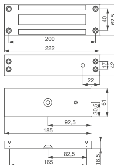
➤ EMSS1200
