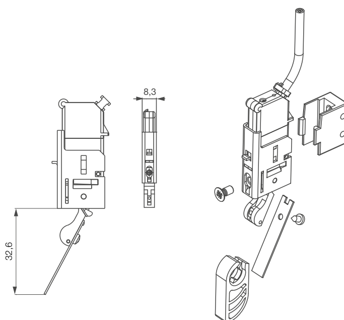
➤ BMK100C
