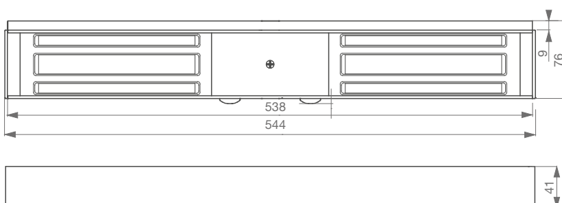
➤ EMS1200CD
