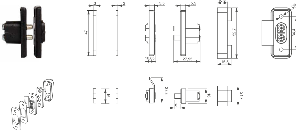
➤ PCT200G
